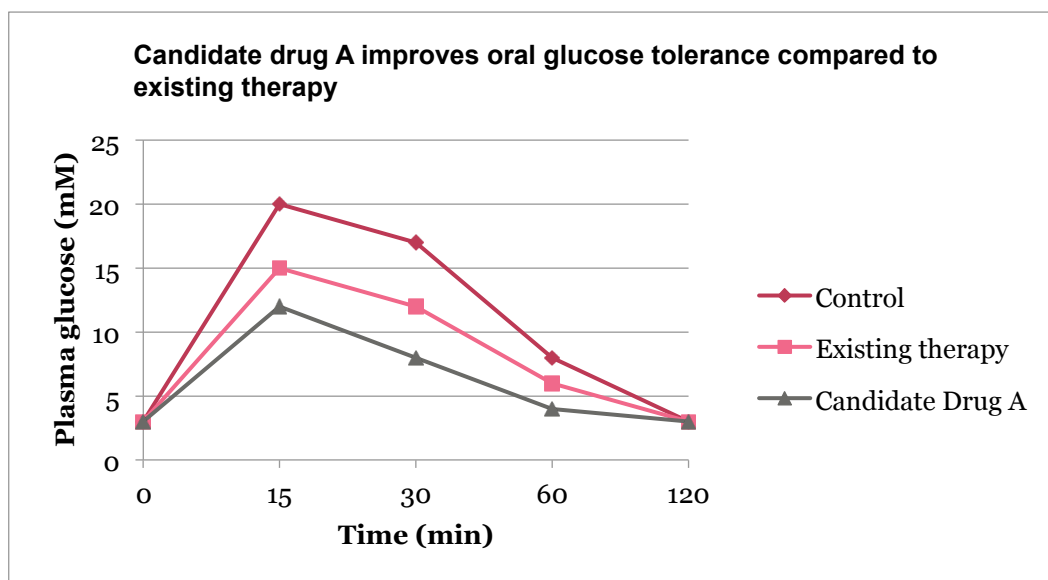
Fig. 1: Plasma concentrations of glucose immediately before and 15, 30, 60, and 120 min after administration of glucose, through gastric gavage in overnight fasted female C57BL6 mice treated with existing anti-diabetic therapy, or novel candidate drug A (Gunnarsson et al., unpublished data).
